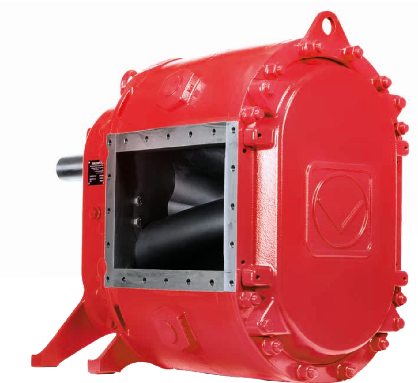
Rotary lobe pumps from the VX series
