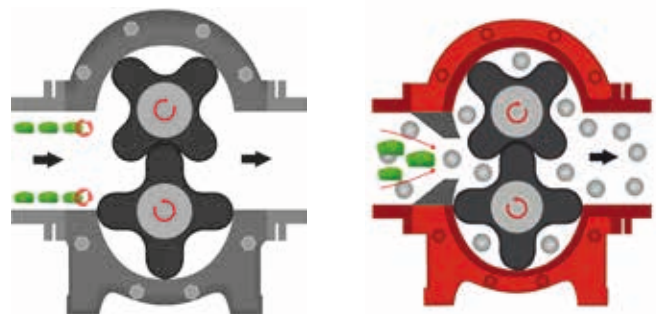
A vortex forms upstream from the inlet in rotary lobe pumps of conventional design. Foreign matter that damages the lobe tips becomes trapped here.
